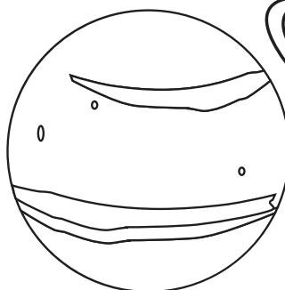
Neptune
