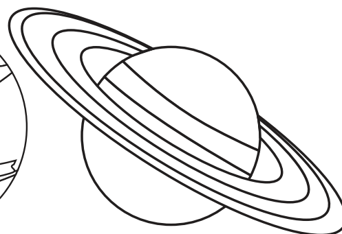
Saturn
